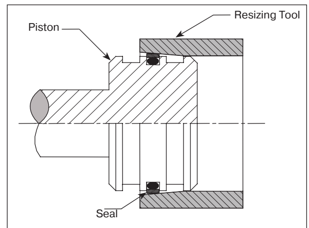
Figure 2-21. Resizing
