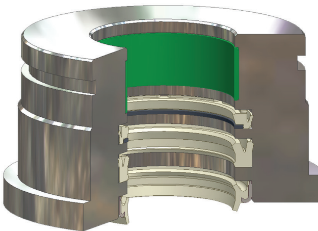
BT Installed in Rod Gland
