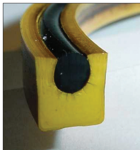
Figure 2-9. Seal exhibiting nearly 100% compression set
