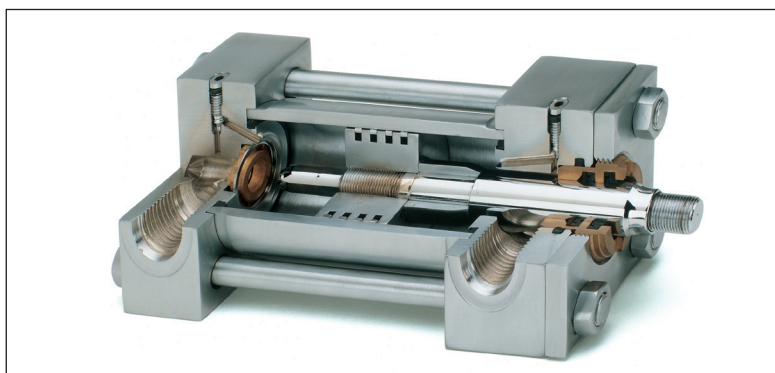
Fig. 2-1. Hydraulic cylinder
