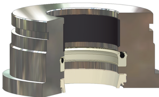
YD installed in Rod Gland
