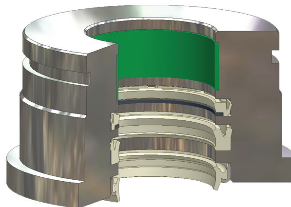
BR Installed in Rod Gland
