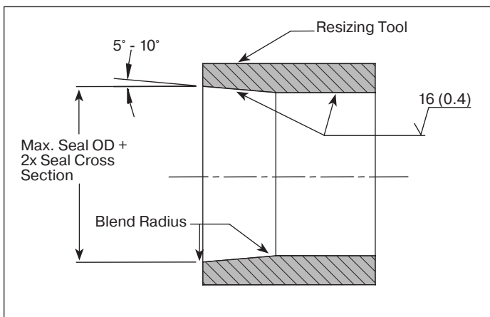
Figure 2-20. Resizing tool
