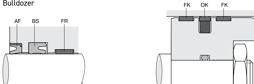
Bulldozer
