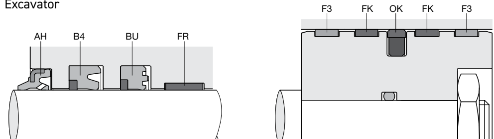
Excavator
