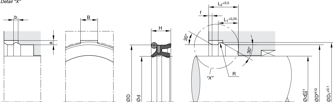
Detail "X"
