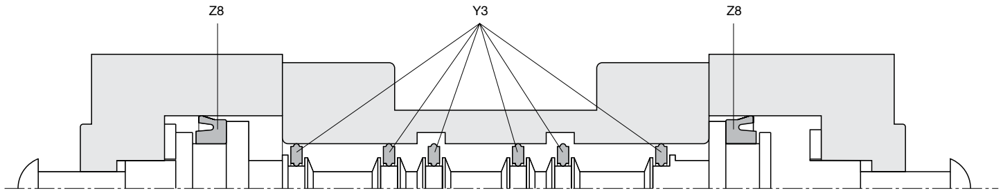
Spool valve
