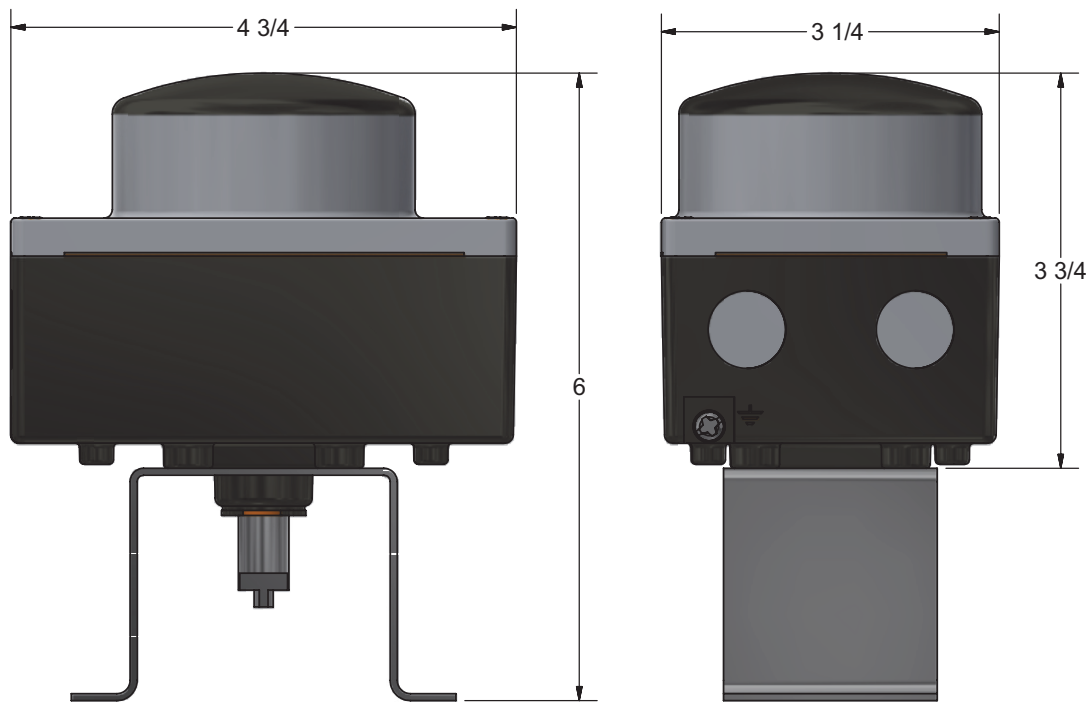
SB Limit Switch
