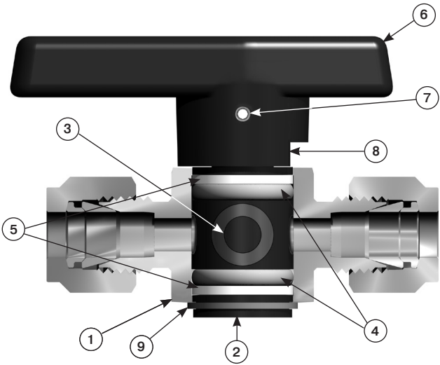
Model Shown: 4A-PR4-VT-SS
