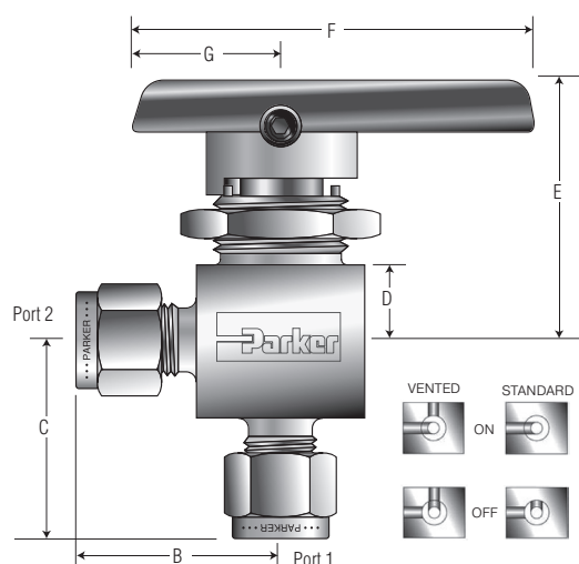
Model shown: 4A-MB6APFA-SSP
