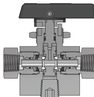
HB4L (Two-Way) Design
