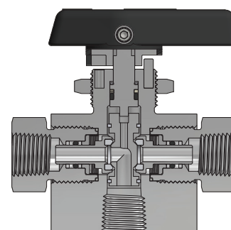
HB4X (Three-Way) Design
