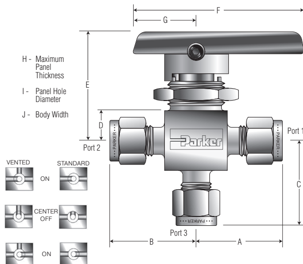
Model shown: 4A-MB6XPFA-SSP
