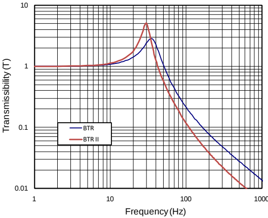
FIGURE 2 – TRANSMISSIBILITY VS. FREQUENCY
