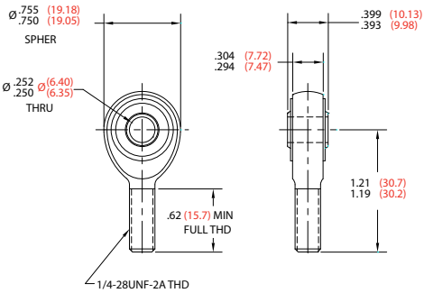
FIGURE 1 – RA-75-3-X PART DIMENSIONS
