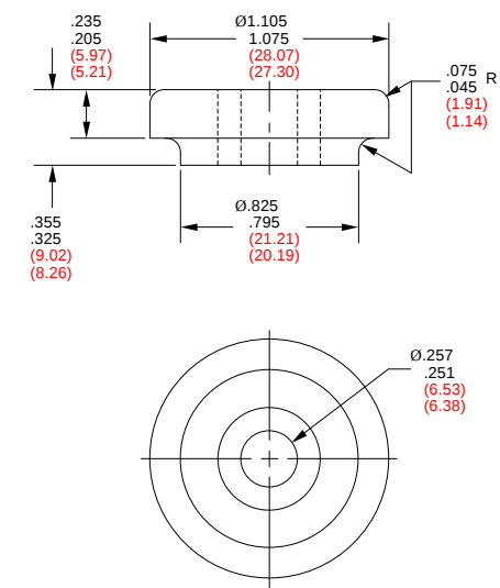
FIGURE 1 – PART DIMENSIONS
