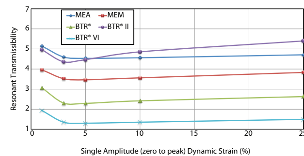
FIGURE 6 – TYPICAL RESONANT TRANSMISSIBILITY VALUES FOR LORD VIBRATION ISOLATOR ELASTOMERS
