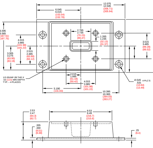
FIGURE 4 – J-18103 PART DIMENSIONS
