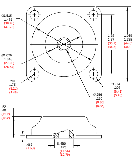
FIGURE 1 – PART DIMENSIONS
