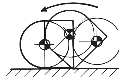
TEST 9 – TIP OVER TEST
