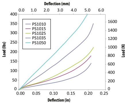
FIGURE 2 – STATIC LOAD VS. DEFLECTION
