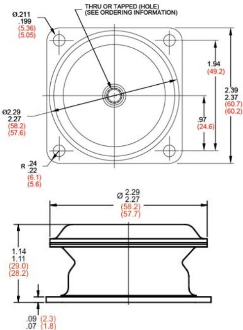
FIGURE 1 – PART DIMENSIONS
