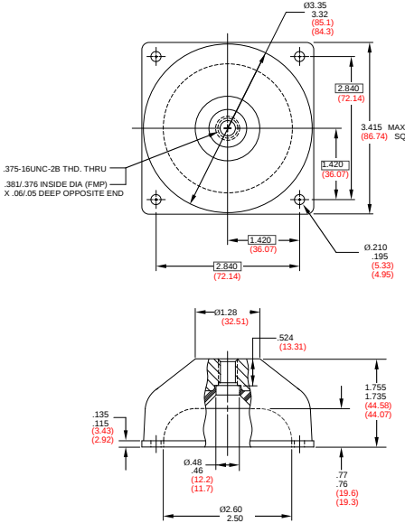
FIGURE 1 – PART DIMENSIONS
