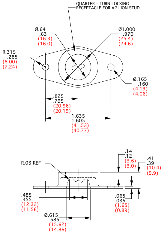
FIGURE 1 – PART DIMENSIONS
