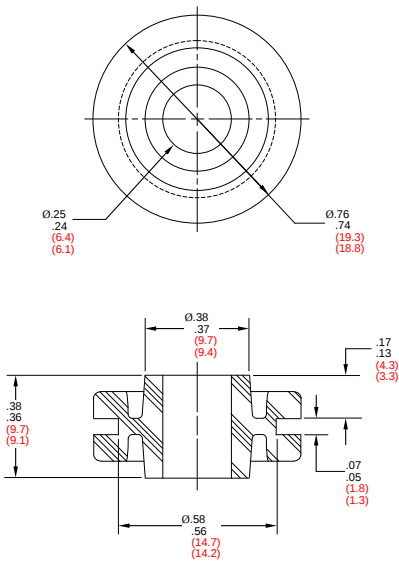
FIGURE 1 – PART DIMENSIONS WITHOUT FERRULE
