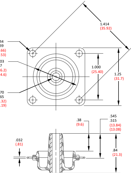
FIGURE 1 – PART DIMENSIONS
