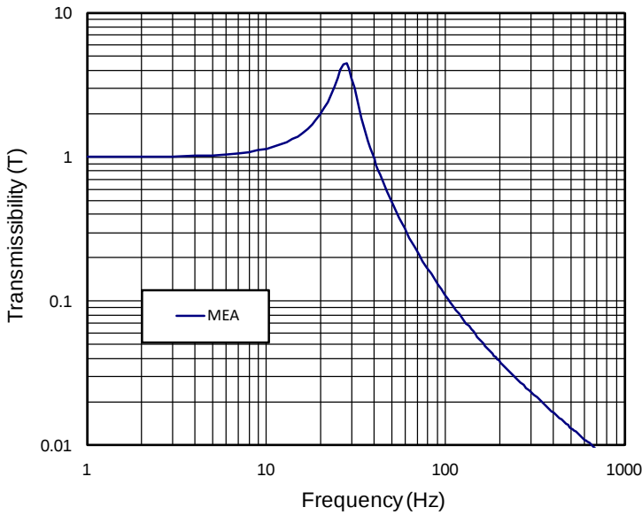
FIGURE 2 – TRANSMISSIBILITY VS. FREQUENCY
