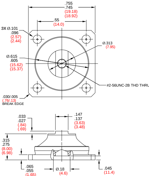
FIGURE 1 – PART DIMENSIONS
