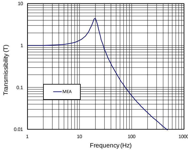
FIGURE 2 – TRANSMISSIBILITY VS. FREQUENCY
