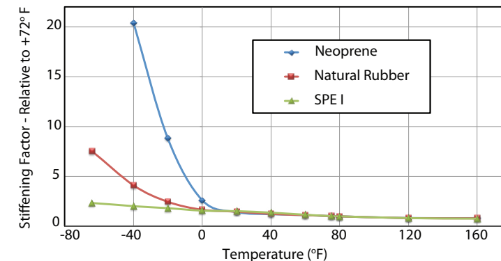
FIGURE 33 – DYNAMIC STIFFNESS OF ELASTOMERS VS. TEMPERATURE
