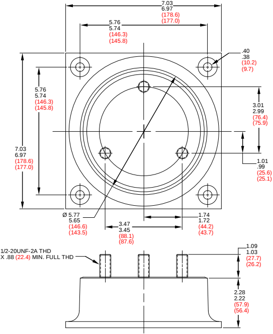
FIGURE 6 – J-18105 PART DIMENSIONS
