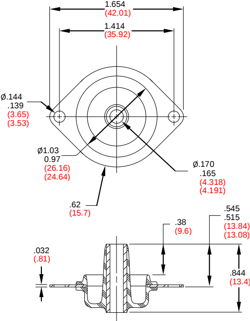
FIGURE 1 – PART DIMENSIONS
