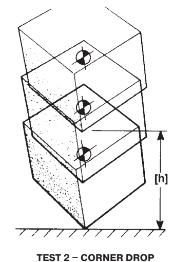
TEST 2 – CORNER DROP
