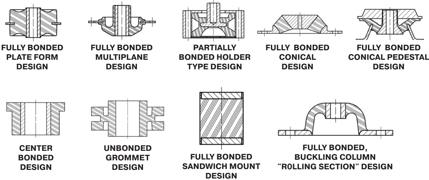
FIGURE 17 – TYPICAL MOUNTING TYPES
