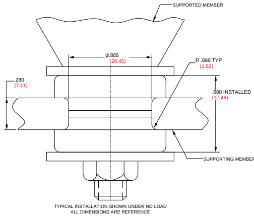
FIGURE 2 – INSTALLATION DRAWING
