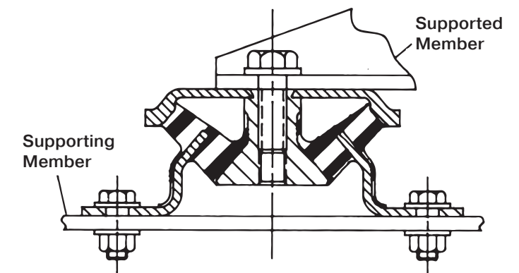
FIGURE 1 – TYPICAL INSTALLATION
