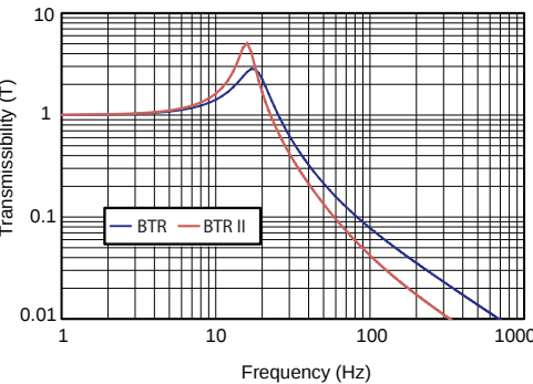
FIGURE 2 – TRANSMISSIBILITY VS. FREQUENCY
