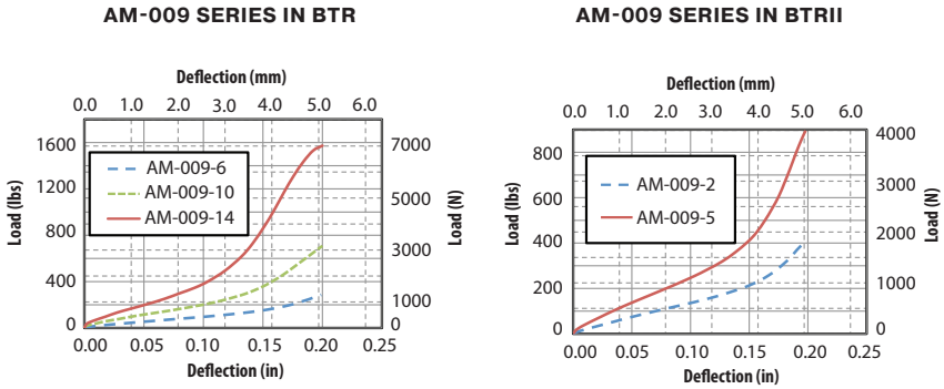
FIGURE 3 – TYPICAL STATIC LOAD VS. DEFLECTION
