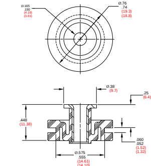
FIGURE 2 – PART DIMENSIONS WITH PLAIN FERRULE
