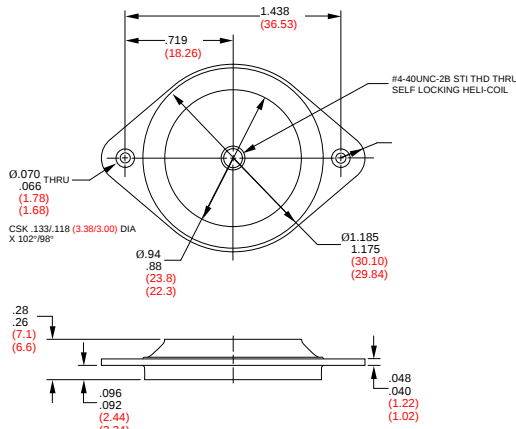
FIGURE 1 – PART DIMENSIONS
