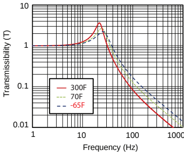
FIGURE 2 – TRANSMISSIBILITY VS. FREQUENCY
