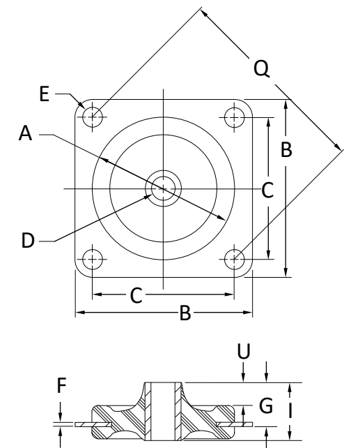
FIGURE 1 – PART DIMENSIONS
