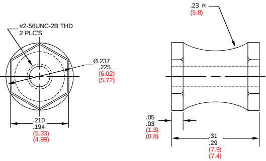
FIGURE 1 – PART DIMENSIONS
