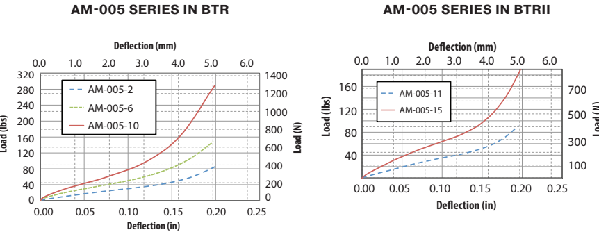
FIGURE 3 – TYPICAL STATIC LOAD VS. DEFLECTION
