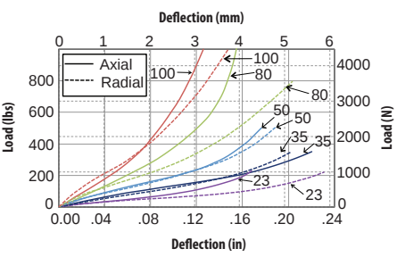
FIGURE 4 – STATIC LOAD VS. DEFLECTION
