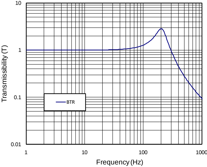
FIGURE 3 – TRANSMISSIBILITY VS. FREQUENCY
