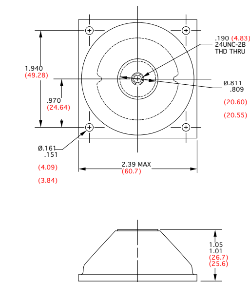
FIGURE 1 – PART DIMENSIONS
