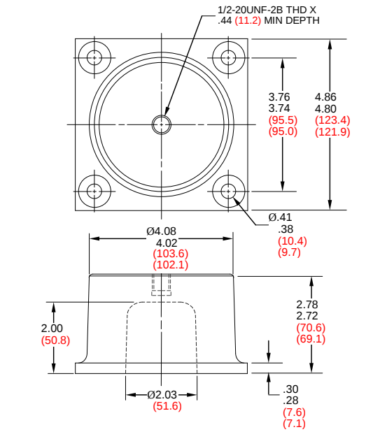
FIGURE 5 – J-18104 PART DIMENSIONS
