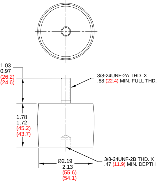
FIGURE 7 – J-18106 PART DIMENSIONS
