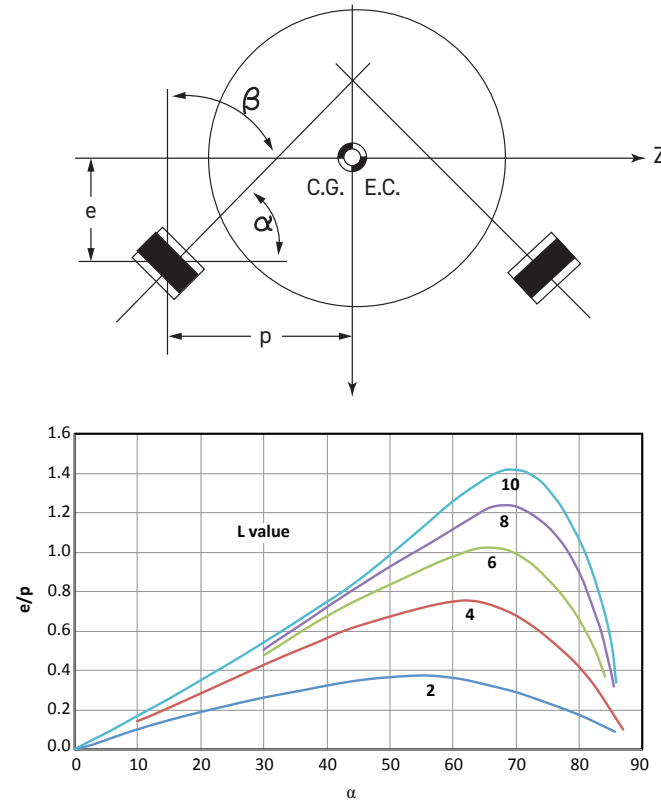
FIGURE 40 – CALCULATION OF FOCALIZATION ANGLE TO PROJECT ELASTIC CENTER TO POINT OF C.G. TO UNCOUPLE SYSTEM
