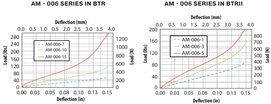
FIGURE 3 – TYPICAL STATIC LOAD VS. DEFLECTION
