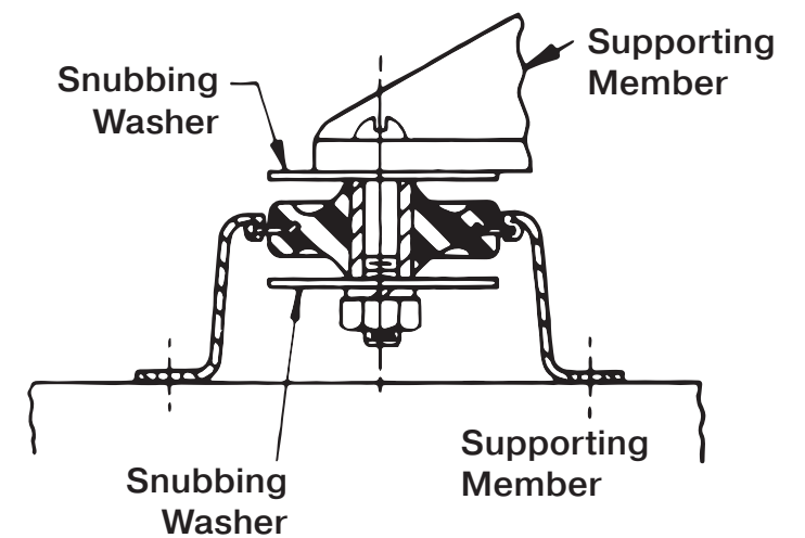
FIGURE 1 – TYPICAL INSTALLATION
