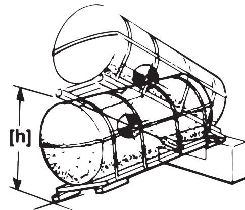
TEST 6 – CORNERWISE ROTATIONAL DROP
