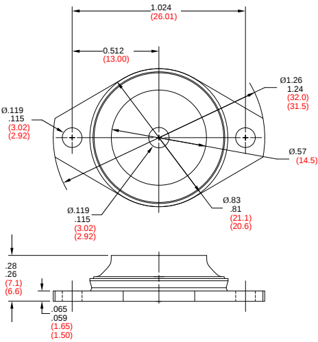
FIGURE 1 – PART DIMENSIONS
