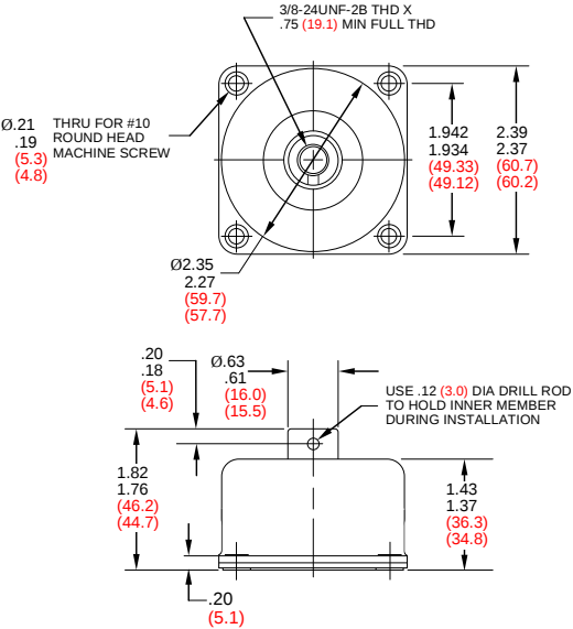
FIGURE 1 – HT2 SERIES PART DIMENSIONS
