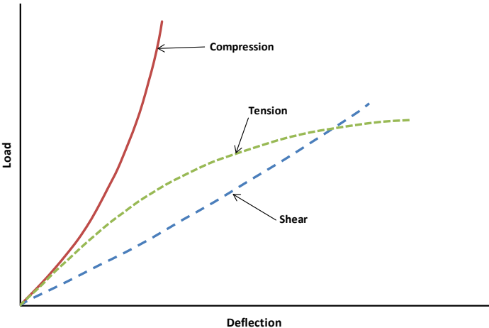
FIGURE 16 – TYPICAL LOAD / DEFLECTION CURVES FOR “SANDWICH” MOUNTS
