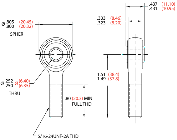
FIGURE 2 – RA-90-9-X PART DIMENSIONS
