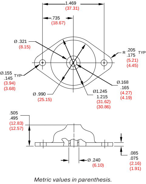
FIGURE 1 – PART DIMENSIONS
