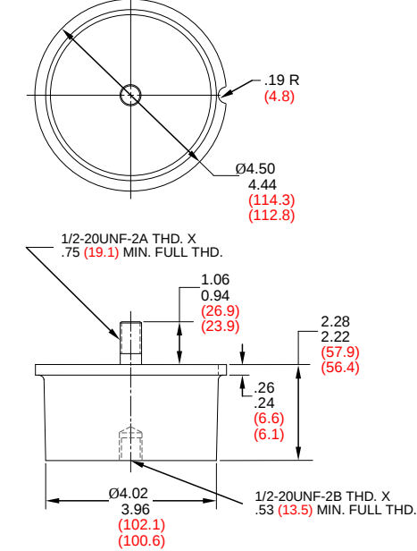
FIGURE 2 – J-18101 PART DIMENSIONS
