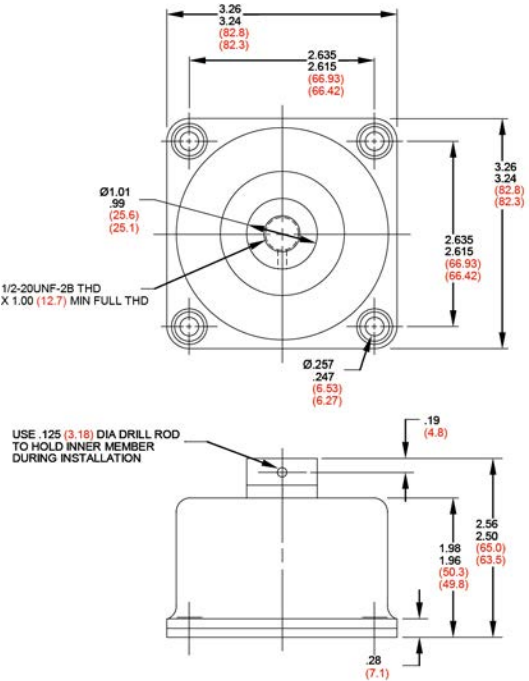
FIGURE 1 – HTC SERIES PART DIMENSIONS
