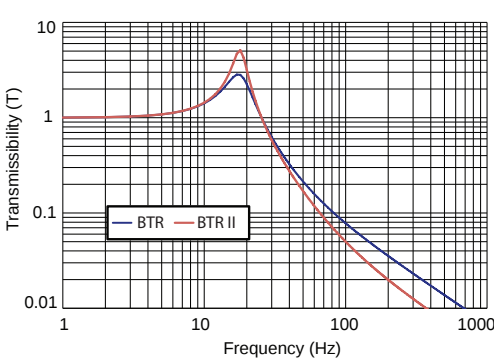
FIGURE 2 – TRANSMISSIBILITY VS. FREQUENCY
