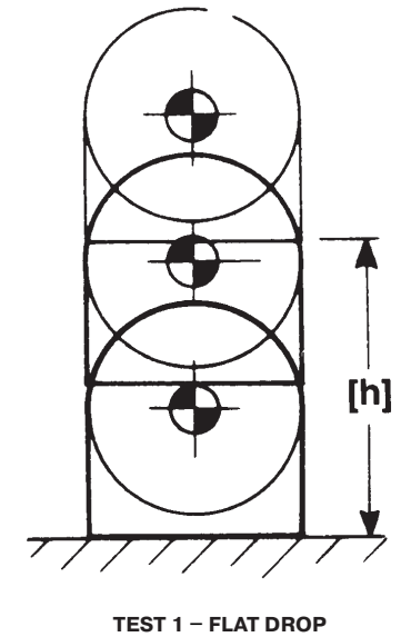
TEST 1 – FLAT DROP
