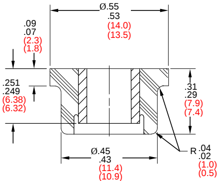
FIGURE 1 – PART DIMENSIONS
