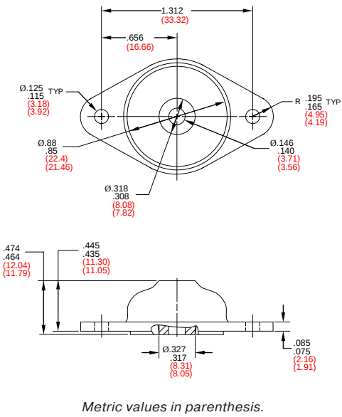
FIGURE 1 – PART DIMENSIONS
