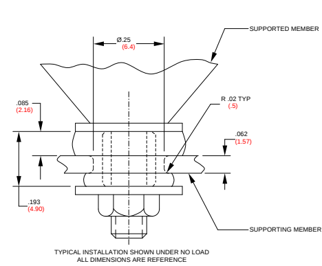
FIGURE 2 – INSTALLATION DRAWING
