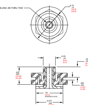
FIGURE 3 – PART DIMENSIONS WITH THREADED FERRULE
