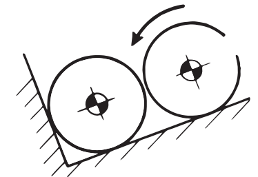
TEST 11 – ROLLING IMPACT TEST (CYLINDRICAL CONTAINERS)
