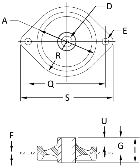
FIGURE 1 – PART DIMENSIONS
