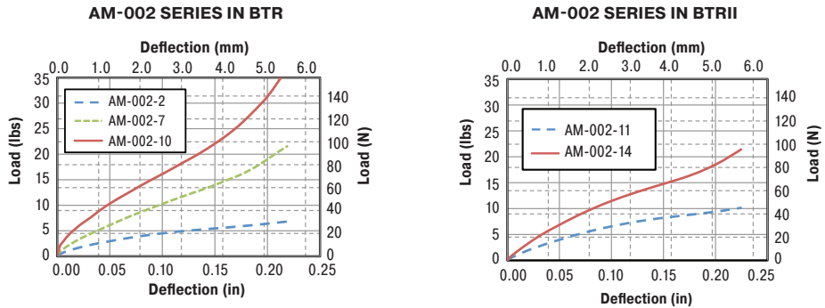
FIGURE 3 – TYPICAL STATIC LOAD VS. DEFLECTION
