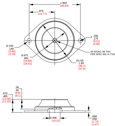
FIGURE 1 – PART DIMENSIONS
