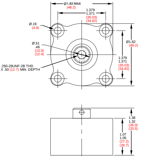
FIGURE 1 – HT1 SERIES PART DIMENSIONS
