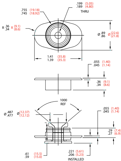
FIGURE 2 – J-23436-8 PART DIMENSIONS
