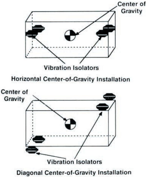
FIGURE 1 – TYPICAL CENTER-OF-GRAVITY INSTALLATIONS
