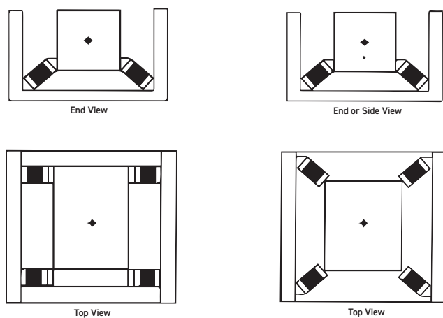
FIGURE 30 – SEMI-FOCALIZED SHIPPING CONTAINER MOUNT SYSTEM
