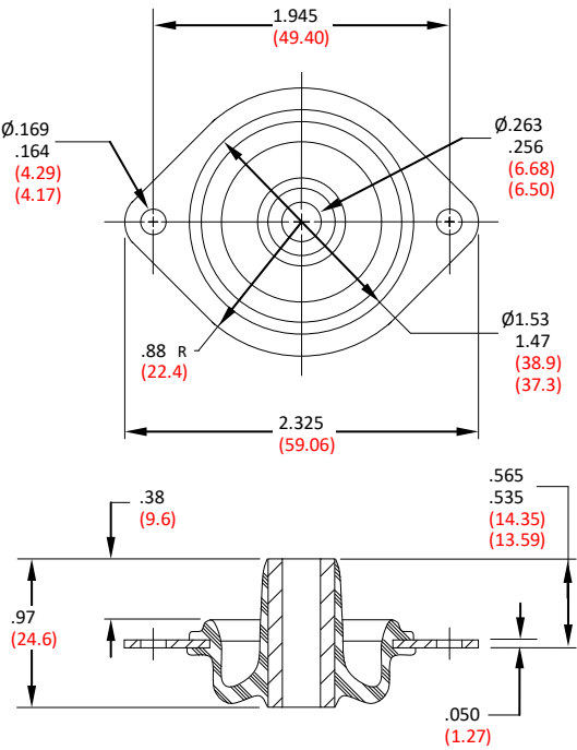
FIGURE 1 – PART DIMENSIONS
