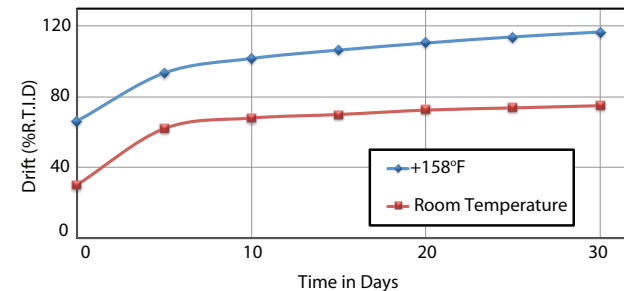
FIGURE 35 – TYPICAL DRIFT CURVE – SPE® I ELASTOMER (30 PSI)
