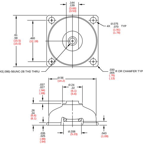
FIGURE 1 – PART DIMENSIONS
