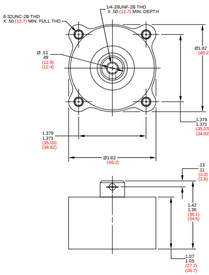
FIGURE 2 – UT1 SERIES PART DIMENSIONS
