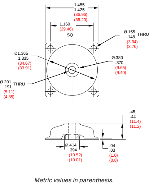
FIGURE 1 – PART DIMENSIONS
