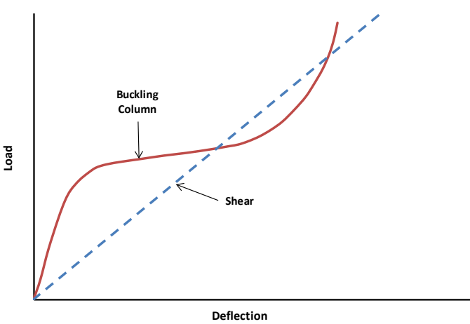
FIGURE 15 – TYPICAL LOAD / DEFLECTION CURVES FOR “ROLLING SECTION” MOUNTS
