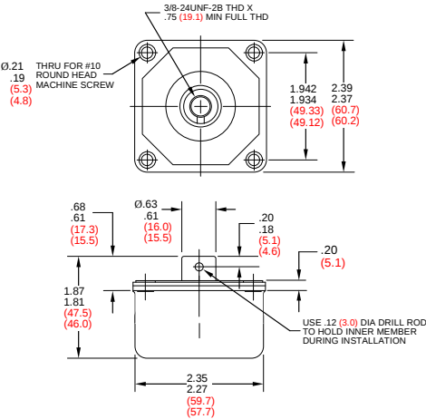
FIGURE 2 – UT2 SERIES PART DIMENSIONS
