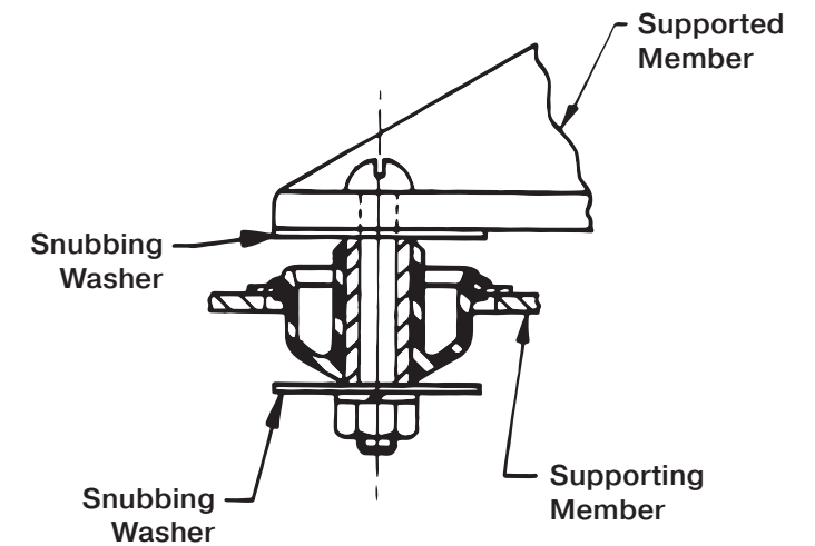
FIGURE 1 – TYPICAL INSTALLATION
