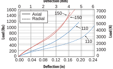
FIGURE 3 – STATIC LOAD VS. DEFLECTION
