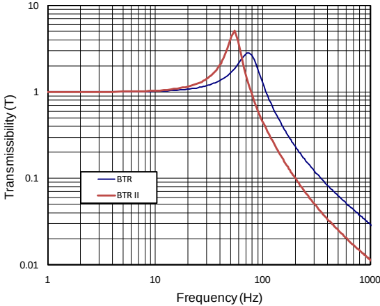
FIGURE 2 – TRANSMISSIBILITY VS. FREQUENCY
