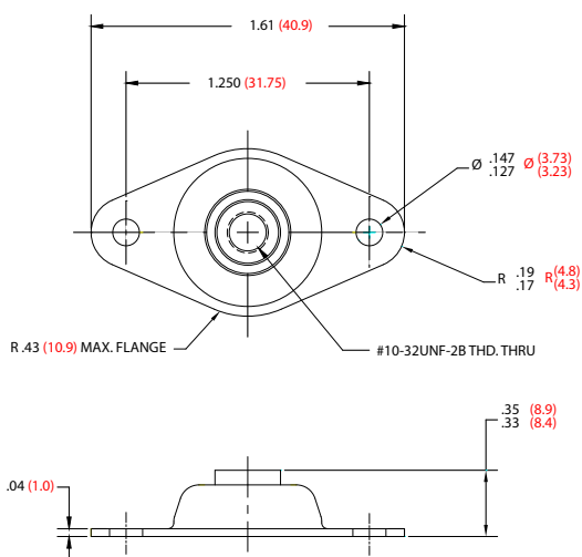
FIGURE 2 – J-23676-1 PART DIMENSIONS
