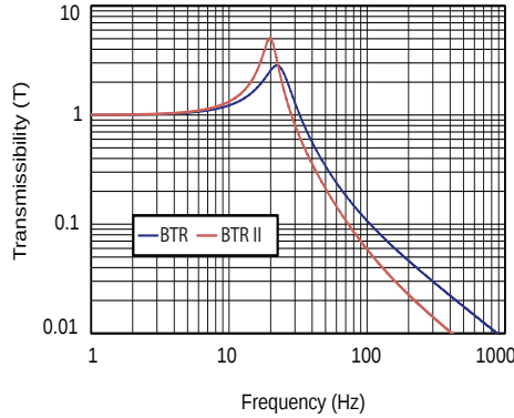
FIGURE 2 – TRANSMISSIBILITY VS. FREQUENCY
