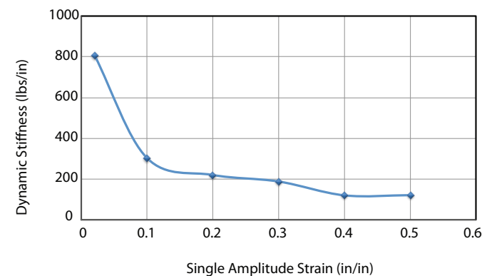
FIGURE 34 – STIFFNESS VS. STRAIN – TYPICAL SPE® I ELASTOMER
