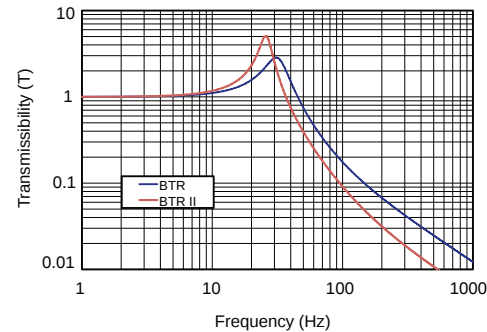
FIGURE 2 – TRANSMISSIBILITY VS. FREQUENCY
