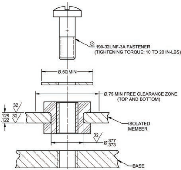
FIGURE 3 – CB-1077-52 INSTALLATION DRAWING
