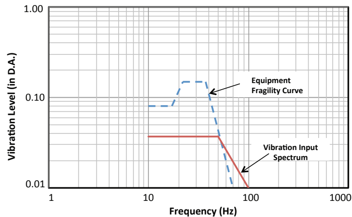
FIGURE 14 – EQUIPMENT FRAGILITY VS. VIBRATION INPUT
