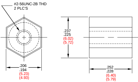
FIGURE 1 – PART DIMENSIONS
