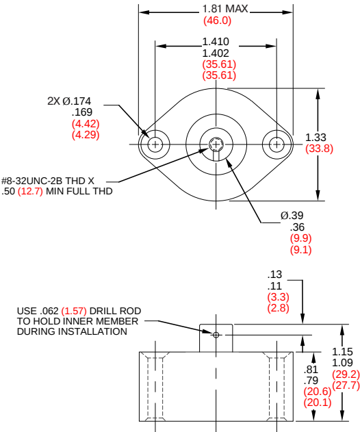
FIGURE 1 – HT0 SERIES PART DIMENSIONS
