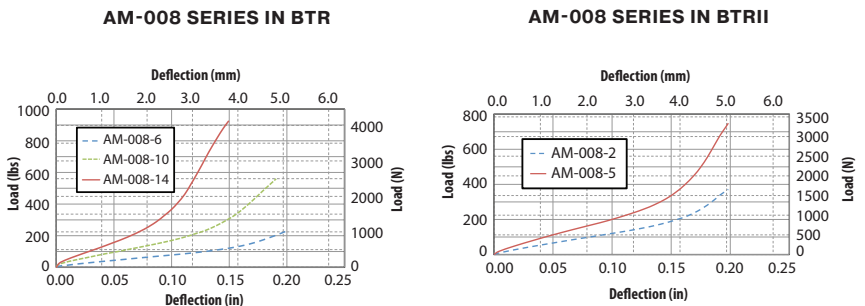
FIGURE 3 – TYPICAL STATIC LOAD VS. DEFLECTION
