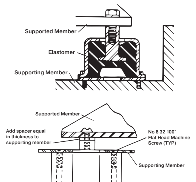
FIGURE 1 – TYPICAL INSTALLATION
