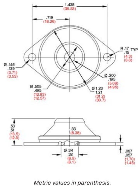
FIGURE 1 – PART DIMENSIONS
