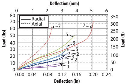
FIGURE 3 – STATIC LOAD VS. DEFLECTION
