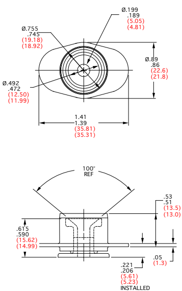
FIGURE 1 – J-23436-7 PART DIMENSIONS
