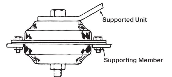
FIGURE 2 – TYPICAL INSTALLATION OF BACK-TO-BACK MOUNT**
