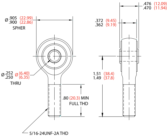
FIGURE 3 – RA-90-10-X PART DIMENSIONS
