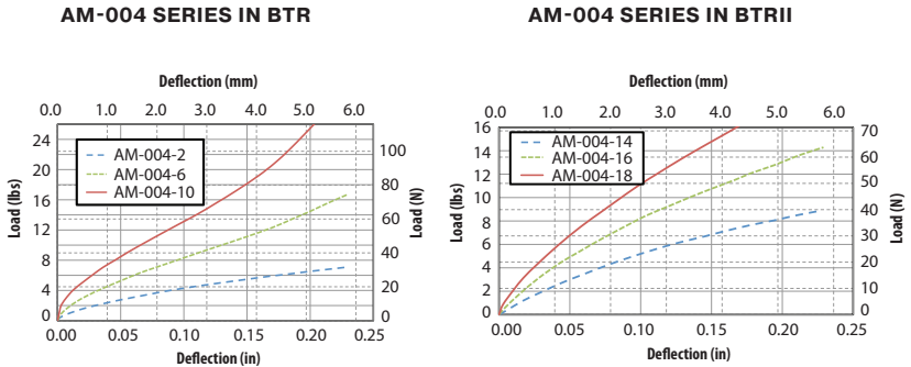
FIGURE 3 – TYPICAL STATIC LOAD VS. DEFLECTION
