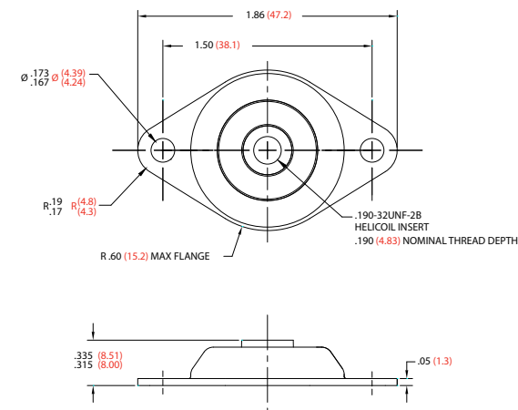
FIGURE 1 – J-23644-3 PART DIMENSIONS
