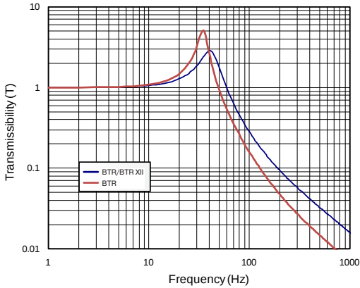
FIGURE 2 – TRANSMISSIBILITY VS. FREQUENCY
