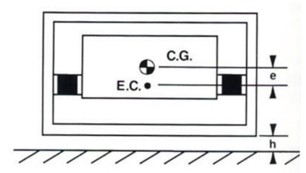
FIGURE 36 – FLAT BOTTOM DROP
