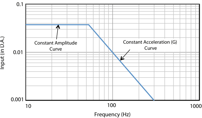
FIGURE 12 – COMPARISON-CONSTANT AMPLITUDE TO CONSTANT “G” VIBRATION INPUT
