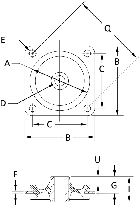
FIGURE 1 – PART DIMENSIONS
