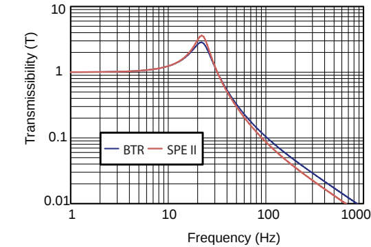
FIGURE 2 – TRANSMISSIBILITY VS. FREQUENCY
