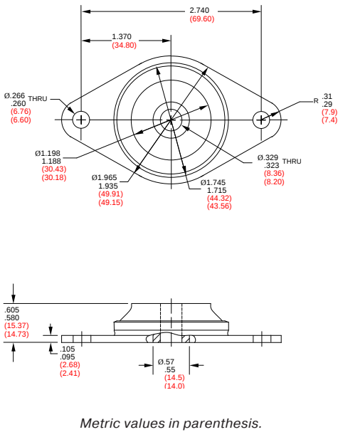
FIGURE 1 – PART DIMENSIONS
