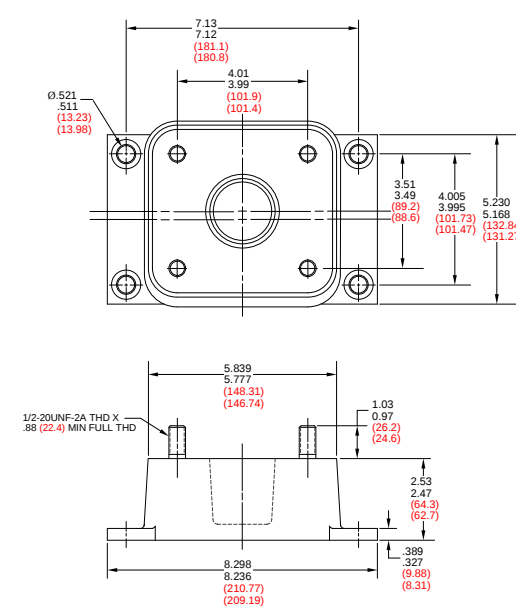
FIGURE 3 – J-18102 PART DIMENSIONS
