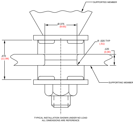
FIGURE 2 – INSTALLATION DRAWING
