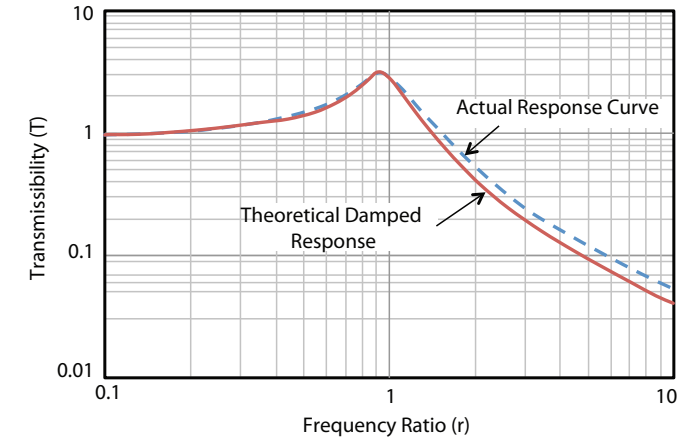
FIGURE 11 – EFFECT OF MATERIAL SENSITIVITY ON TRANSMISSIBILITY RESPONSE
