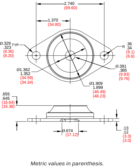
FIGURE 1 – PART DIMENSIONS
