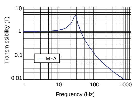
FIGURE 2 – TRANSMISSIBILITY VS. FREQUENCY
