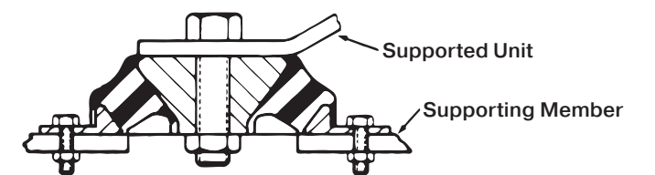
FIGURE 1 – TYPICAL INSTALLATION OF AM SERIES MOUNT*
