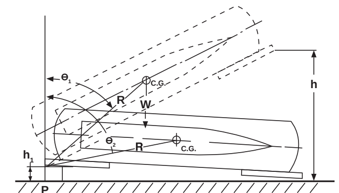
FIGURE 38 - EDGEWISE ROTATIONAL END DROP ANALYSIS
