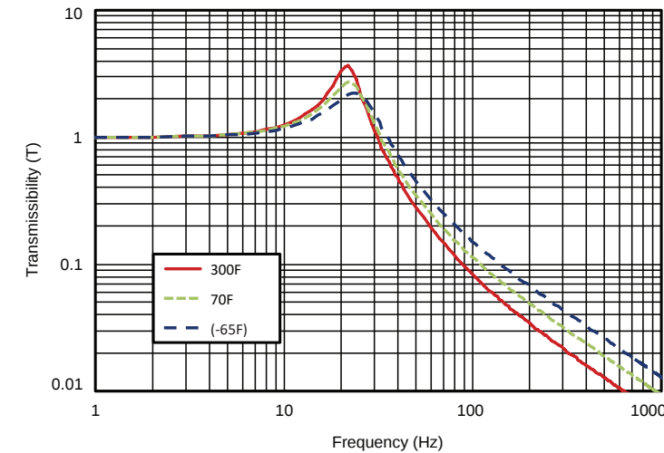
FIGURE 3 – TRANSMISSIBILITY VS. FREQUENCY
