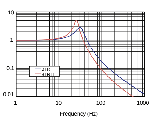
FIGURE 2 – TRANSMISSIBILITY VS. FREQUENCY
