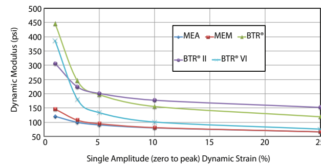
FIGURE 5 – TYPICAL DYNAMIC ELASTIC MODULUS VALUES FOR LORD VIBRATION ISOLATOR ELASTOMERS
