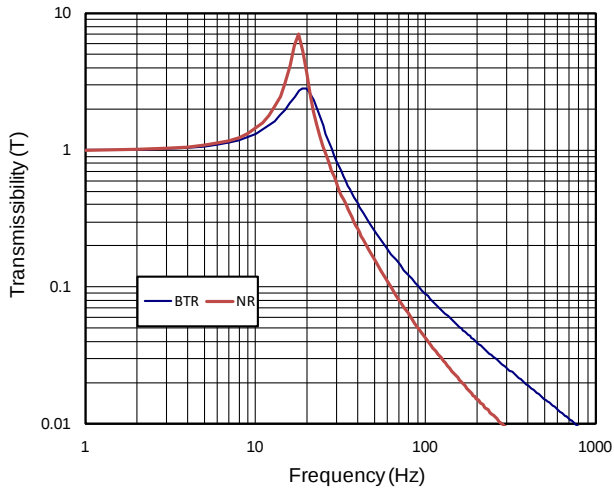
FIGURE 3 – TRANSMISSIBILITY VS. FREQUENCY
