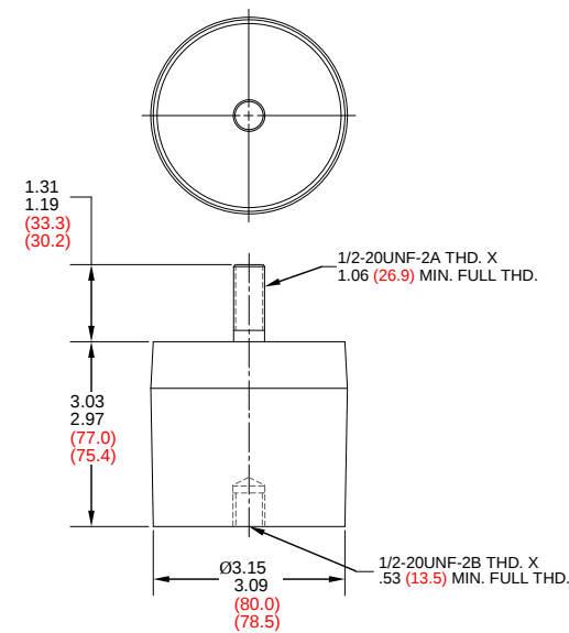
FIGURE 1 – J-18100 PART DIMENSIONS
