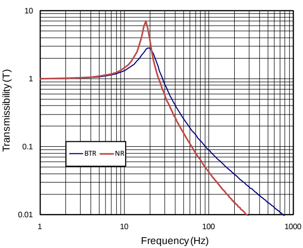
FIGURE 3 – TRANSMISSIBILITY VS. FREQUENCY
