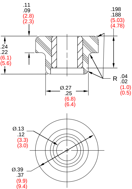
FIGURE 1 – PART DIMENSIONS
