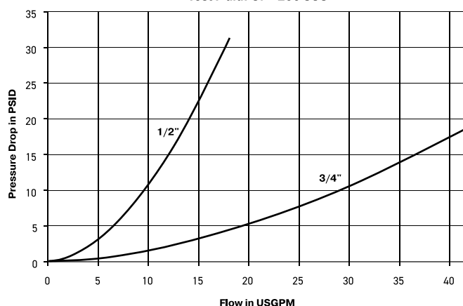
SM Series (1/2" & 3/4") Test Fluid: Oil - 200 SUS
