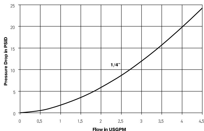
SM Series (1/4") Test Fluid: Oil - 200 SUS
