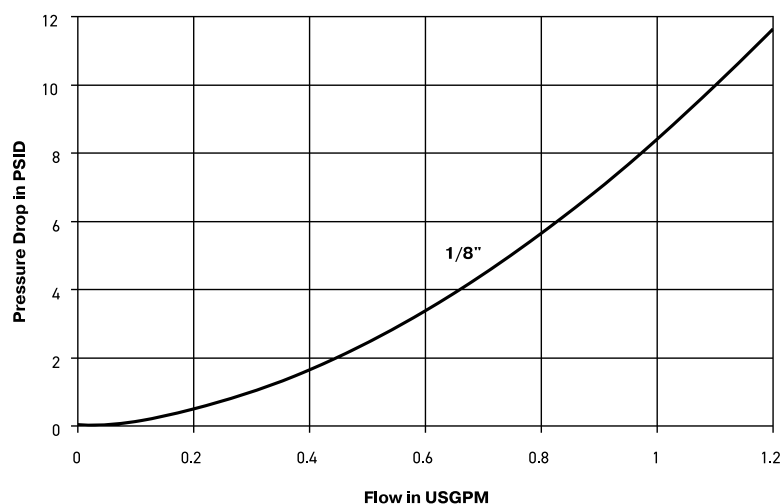
Rectus 21 DSO Series (1/8") Test Fluid: Water
