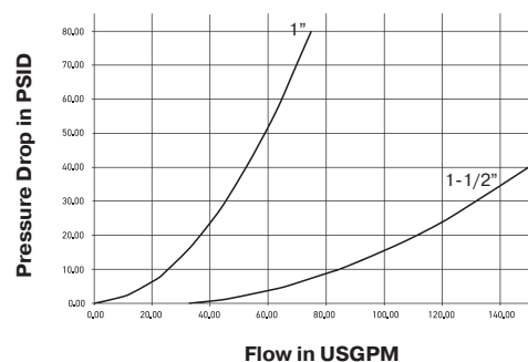
59 Series (1" & 1-1/2") Test Fluid: Oil - 150 SUS)
