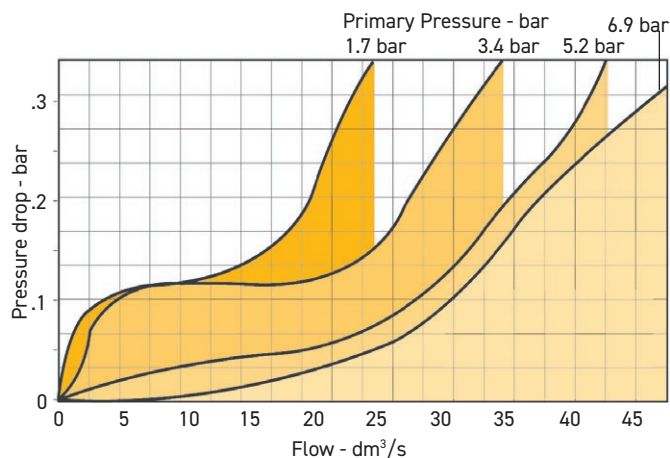
Flow Characteristics - 1/2 Inch Ports PL10-04DSS
