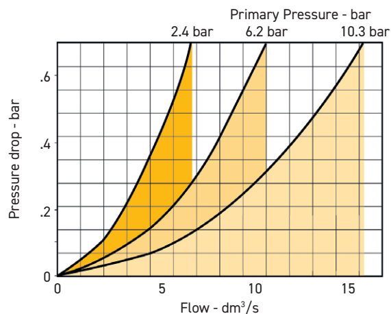
Flow Characteristics - 1/4 Inch Ports PF501-02DHSS
