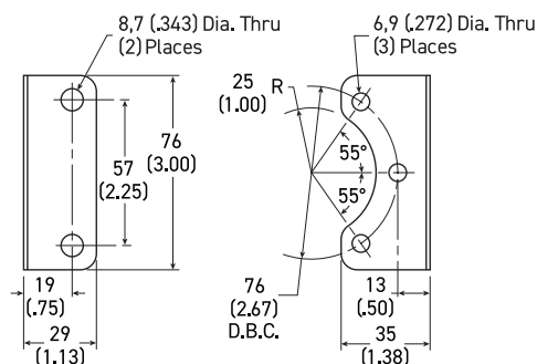
Mounting Bracket 446-707-025
