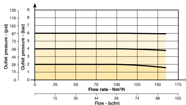
Flow Curve 1/2"
