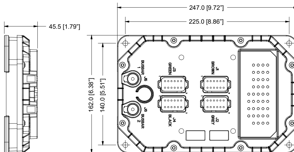
Figure 23: CM2115 dimensions
