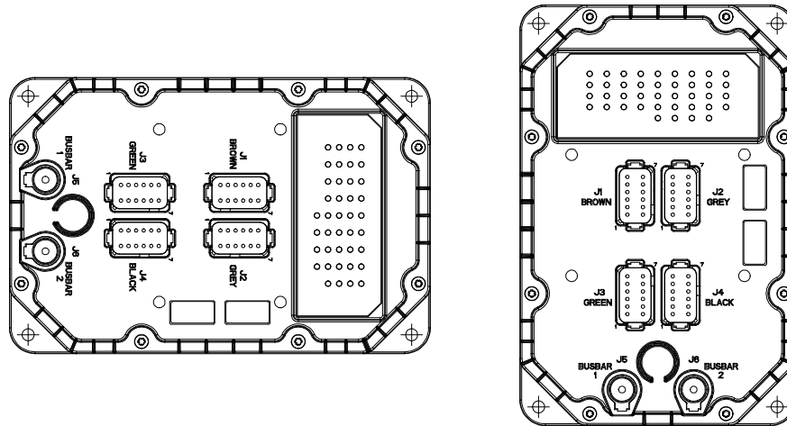
Figure 24: Recommended orientations
