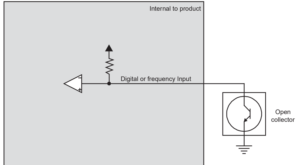
Figure 30: Open collector sensor connection
