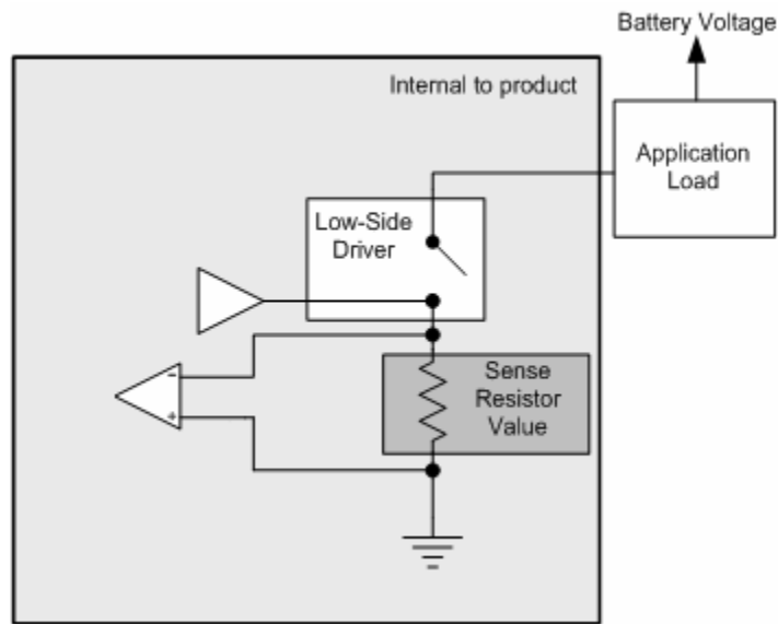
Figure 18: Low-side output with current sense configuration
