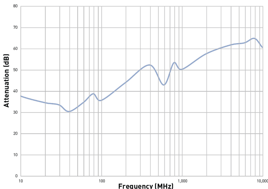
Figure 1 Shielding Effectiveness for CHO-SHRINK 1120, 1/2" diameter tubing
