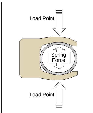
Figure 2-18. Installed State
