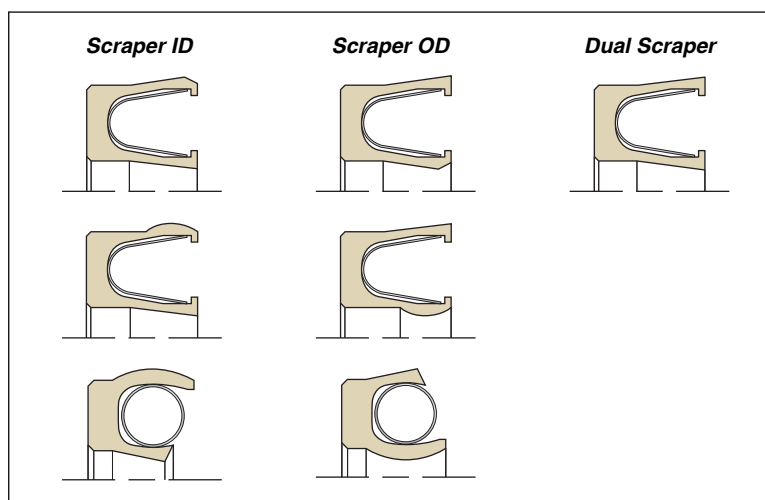
Figure 2-20. Scraper Lips
