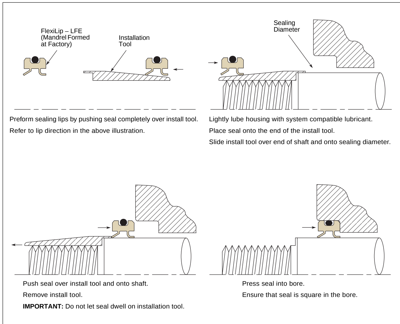
Figure 8-1. FlexiLip Installation
