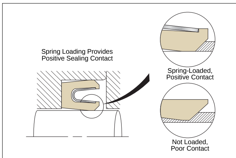
Figure 2-14. Spring Loading
